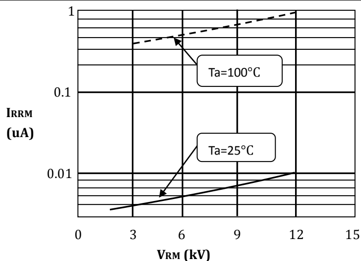
Reverse Characteristics
