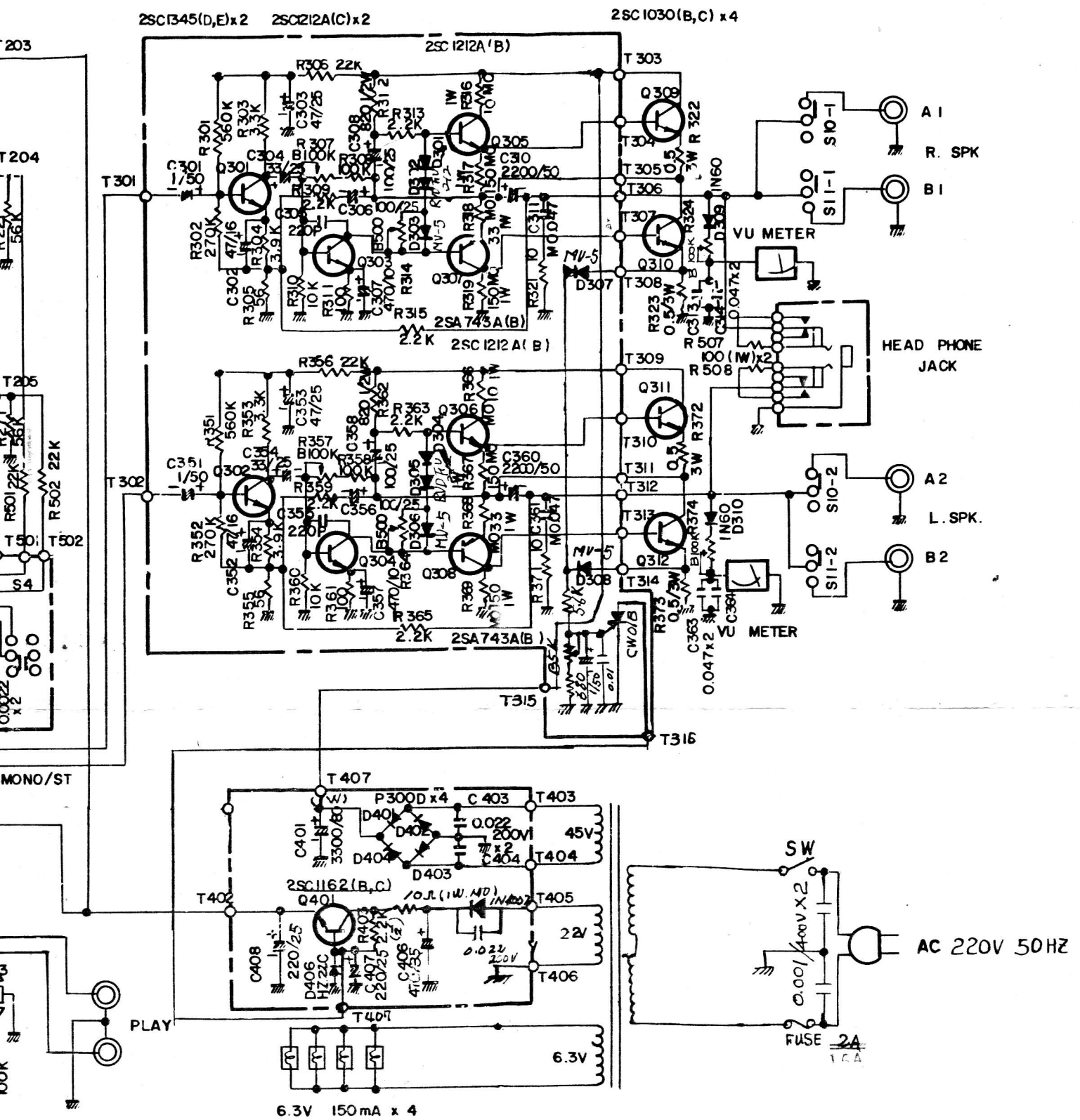
SCHMATIC DIAGRAM FOR MODEL ID-340
