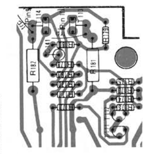
MAIN BOARD SEGMENT LOCATIONS (X-Final Amplifier)
