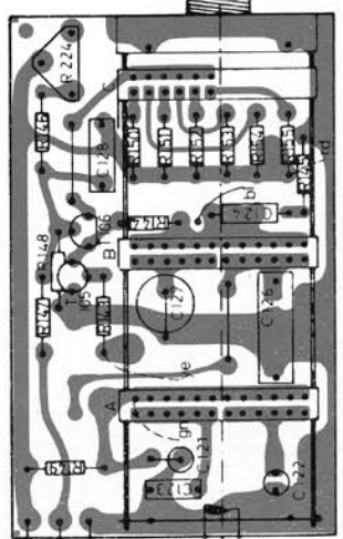
COMPONENT LOCATIONS TIMEBASE SWITCH UNIT
