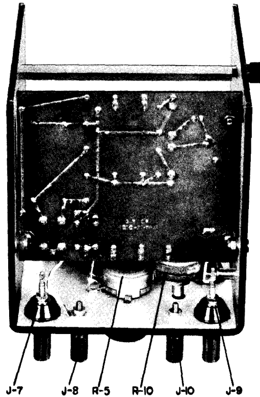
Figure 10. Bottom Interior View of Type 1210-P1 Detector and Discriminator.
