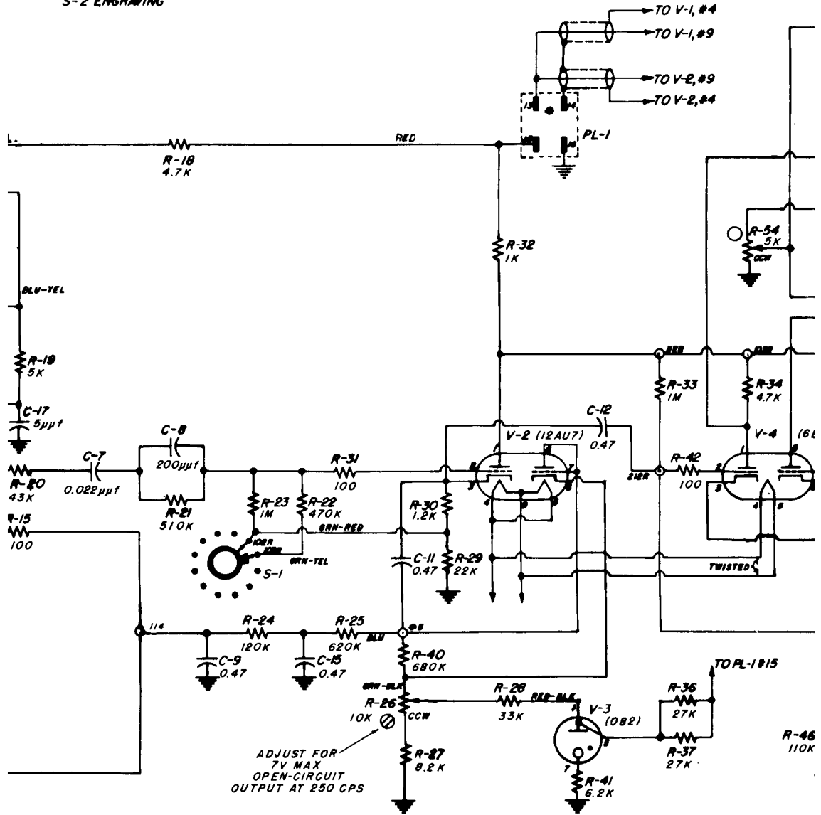
Figure 6. Wiring Diagram for Type 1210-B Unit R-C Oscillator.
