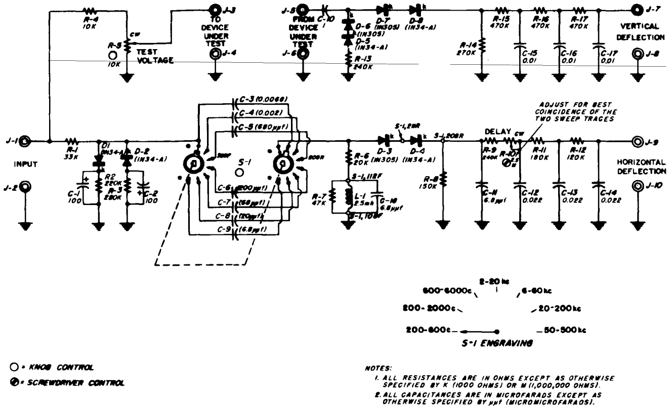
Figure 11. Wiring Diagram for Type 1210-P1 Detector and Discriminator.
