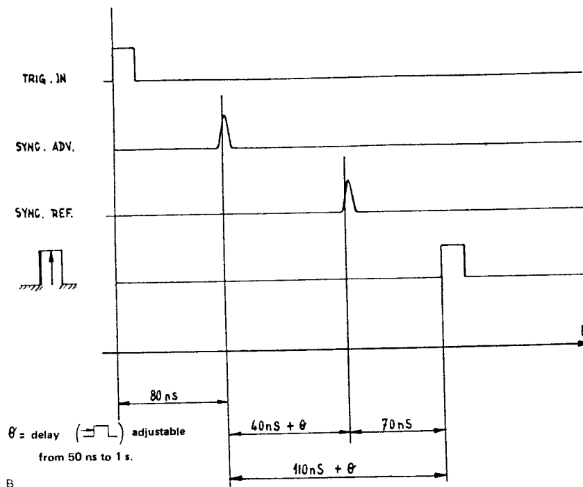
Figure 2 - Waveforms
