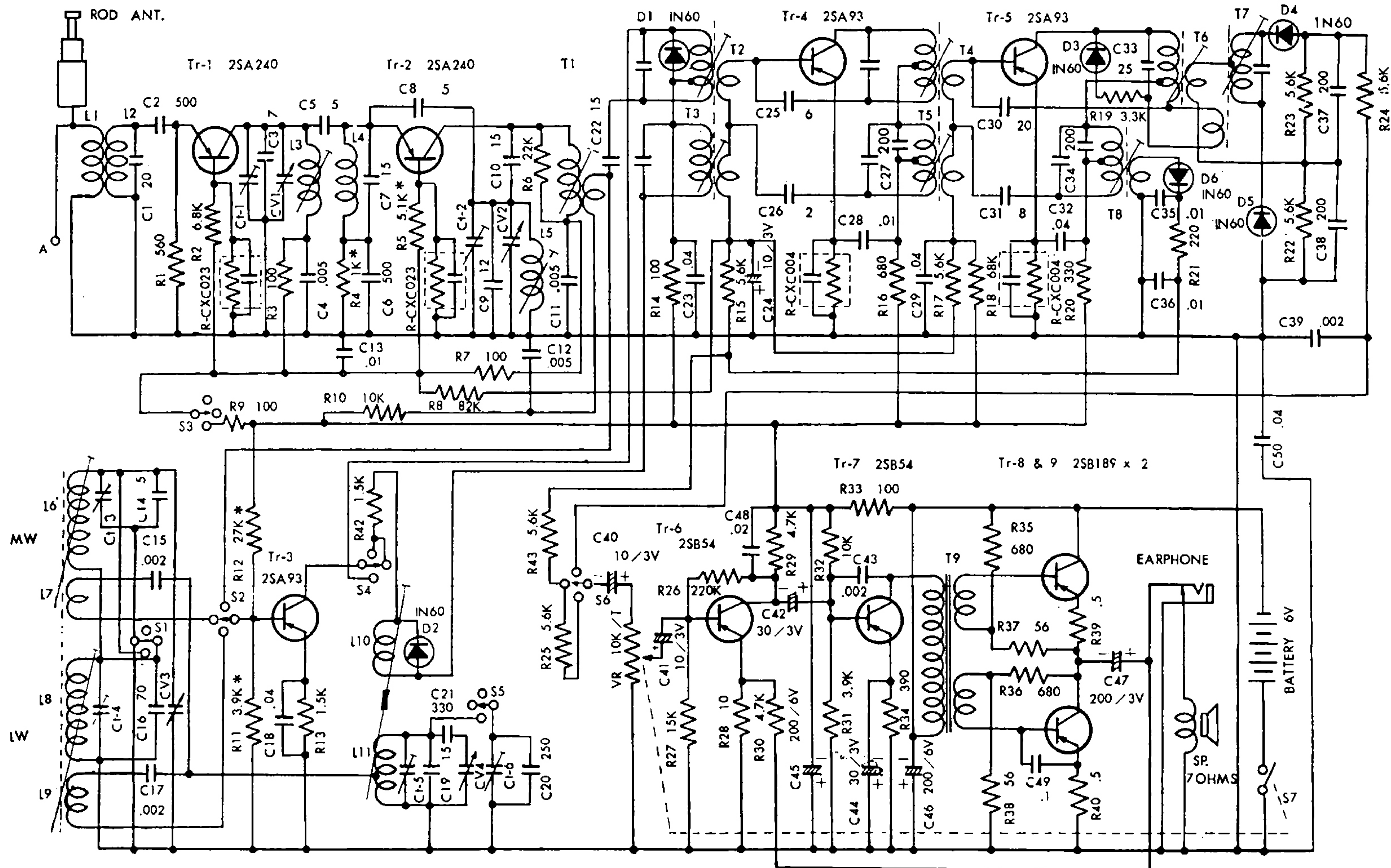
CIRCUIT DIAGRAM—SANYO MODEL AFT-6N
