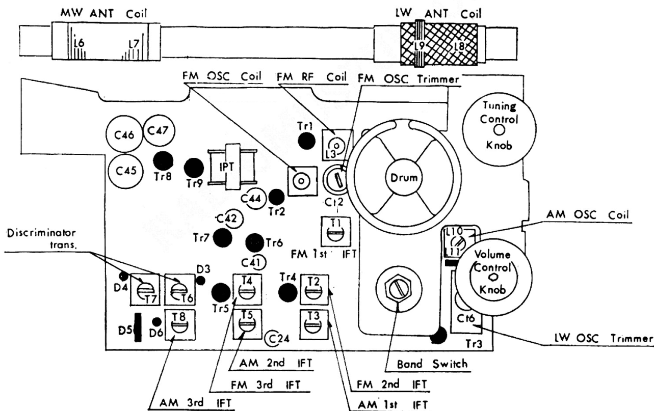
LAY-OUT DIAGRAM—SANYO MODEL AFT-6N
