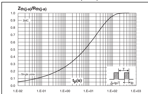
Figure 7. Relative variation of thermal impedance junction to ambient versus pulse duration (SMC)
