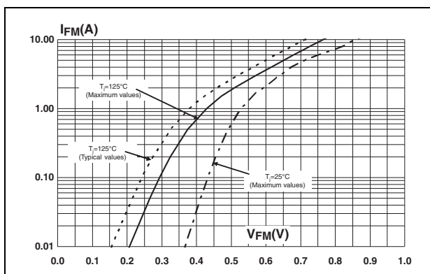
Figure 11. Forward voltage drop vs. forward current
