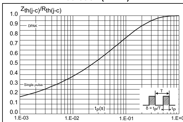
Figure 5. Relative variation of thermal impedance junction to case versus pulse duration (DPAK)
