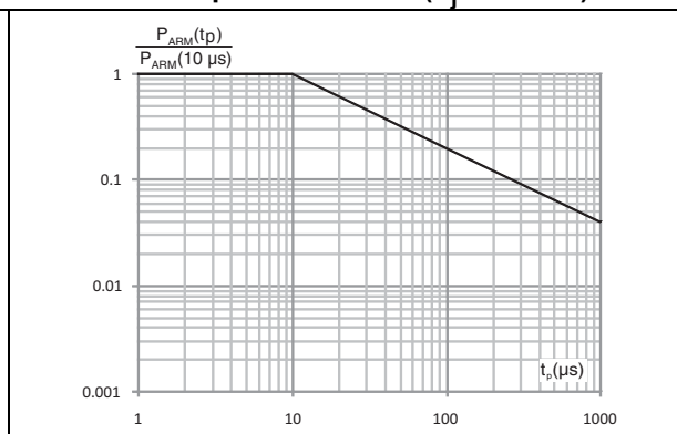
Figure 4. Normalized avalanche power derating versus pulse duration (Tj = 125 C)
